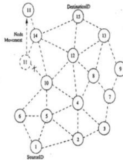
Figure 7.8. Route maintenance in DSDV.
