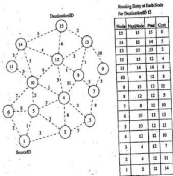
Figure 7.7. Route establishment in WRP.
