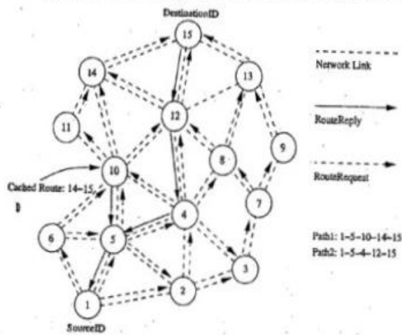
Figure 7.12. Route establishment in AODV.
