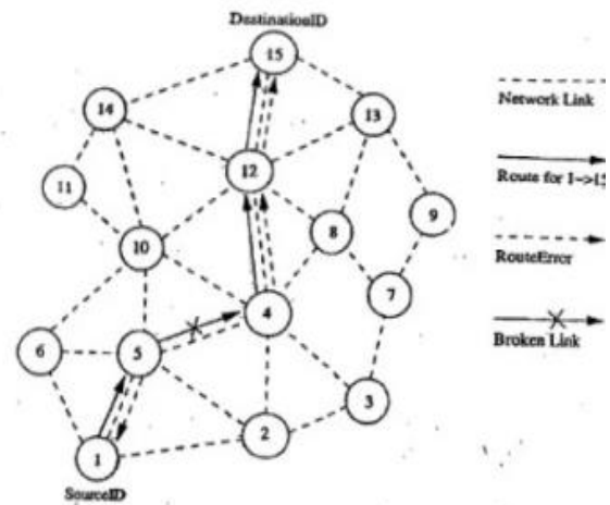
Figure 7.13. Route maintenance in AODV.
