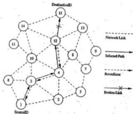
Figure 7.11. Route maintenance in DSR.
