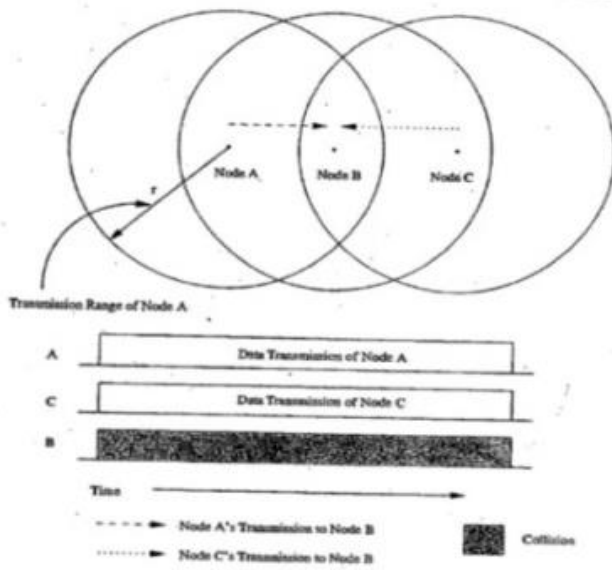
Figure 7.1. Hidden terminal problem.
