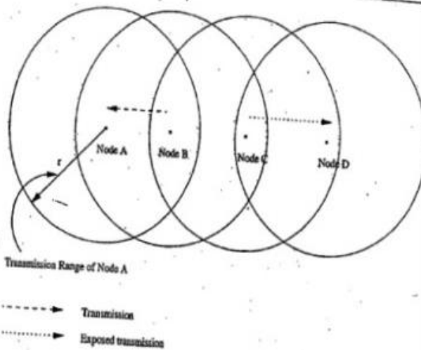
Figure 7.3. Exposed terminal problem.
