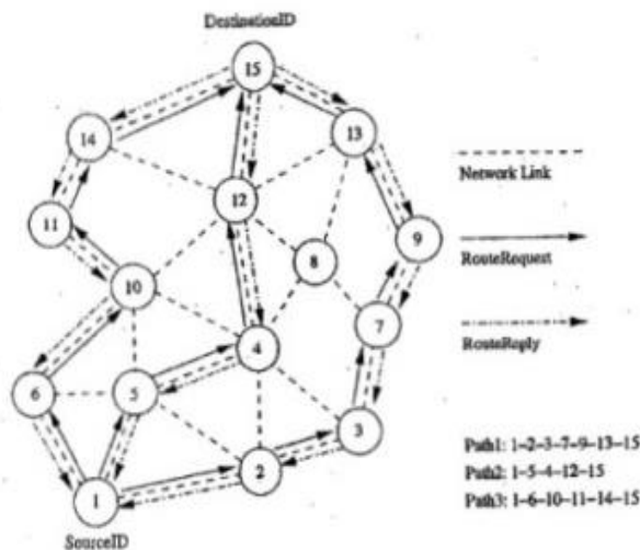
Figure 7.10. Route establishment in DSR.
