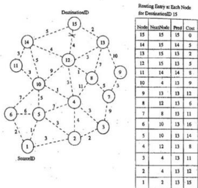
Figure 7.8. Route maintenance in WRP.
