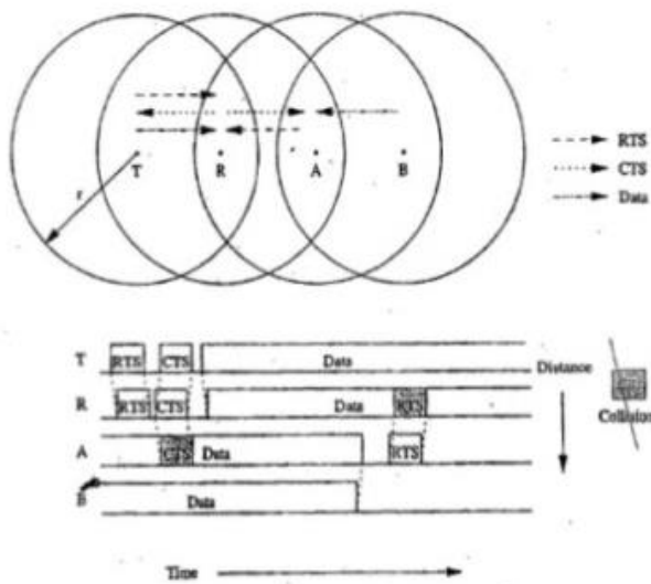
Figure 7.2. Hidden terminal problem with RTS-CTS-Data-ACK scheme.
